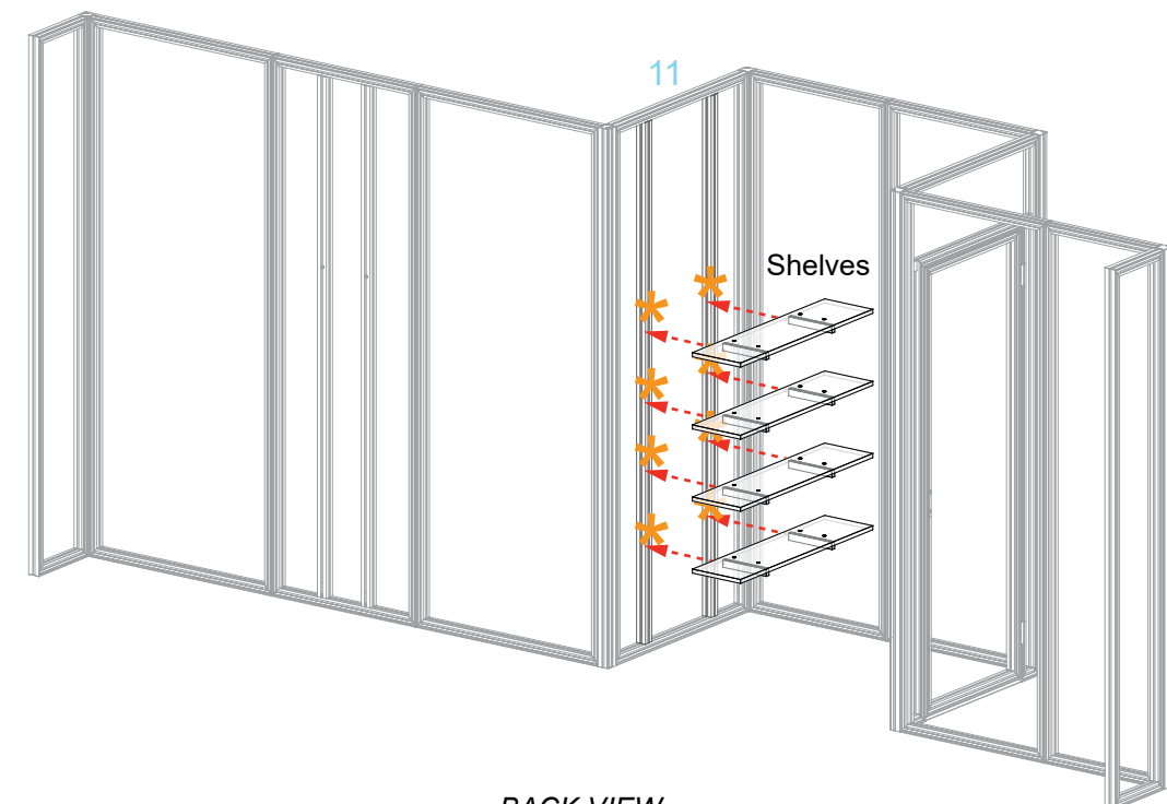
BACK VIEW
